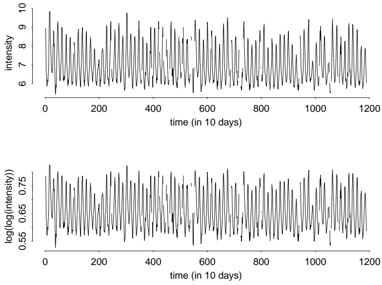
Figure 1: 1189 observations of light intensity from S. Carinae star in both the original units and on a log-log scale.
