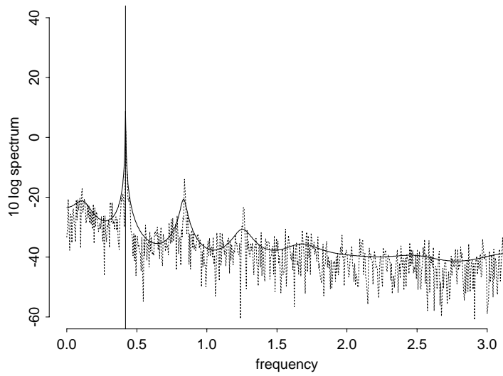
Figure 9: Periodogram of the log-log series ( dashed line ) and the posterior mean for the autoregressive spectrum ( solid line ).
