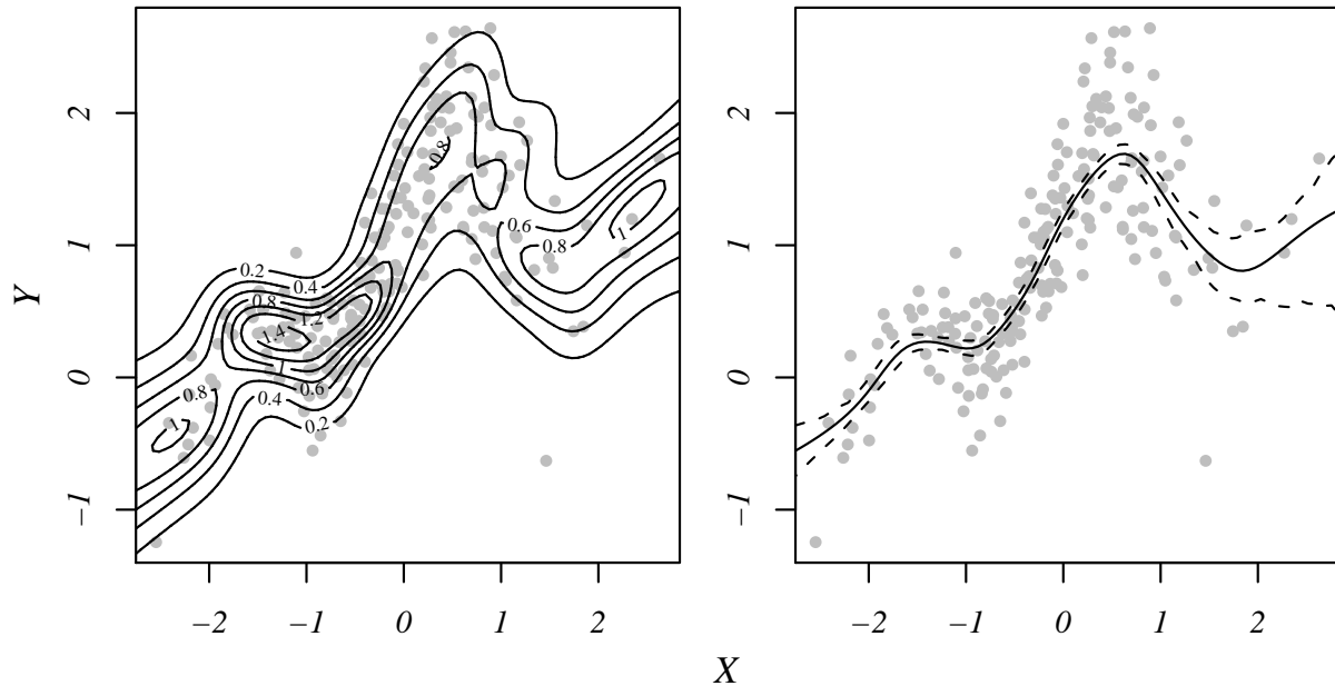
Figure 5: Regression Example. Data and conditional inference for the example of Section 4.3. The left panel shows the filtered posterior mean estimate for the conditional density f(x, y; G_L)/f(x; G_L) , and the right panel shows the posterior mean and 90% interval for the mean \mathbb{E}[y|x; G_L] .
