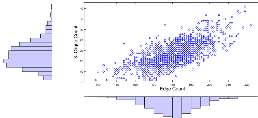
FIG 11. Edge counts and 3-Clique counts from 1000 simulated samples of an Erdős-Rényi graph with edge inclusion probability of p = 0.065 .
