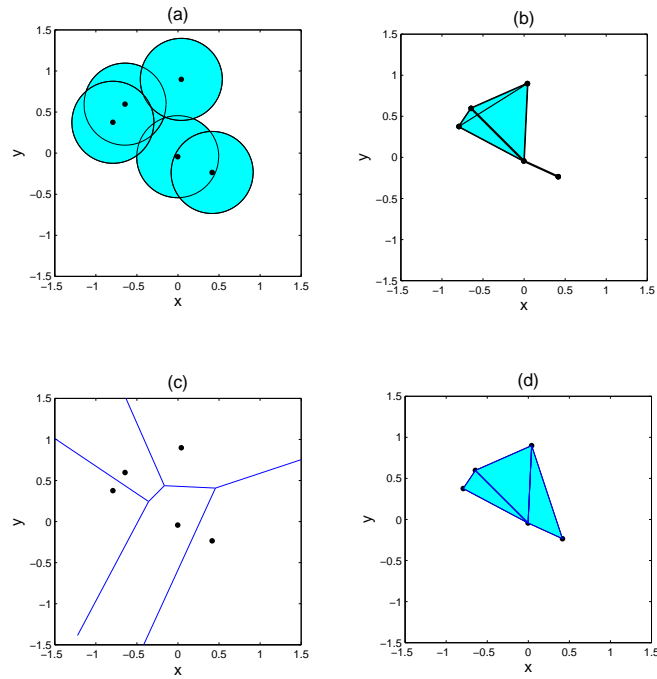
FIG 2. (a) A set of vertices in \mathbb{R}^2 are used to construct a family of disks of radius r = 0.5 . (b) The nerve of this convex set. This is an example of a Čech complex. (c) For the same vertex set the Voronoi diagram is computed. (d) The nerve of the Voronoi cells is obtained. This is an example of the Delaunay triangulation. Note that the maximum clique size of the Delaunay is bounded by the dimension of the space of the vertex set plus one; such a restriction does not apply to the Čech complex.
