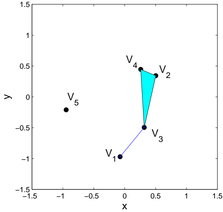
FIG 19. Graph encoding the Markov structure of the model given in (5.5).
