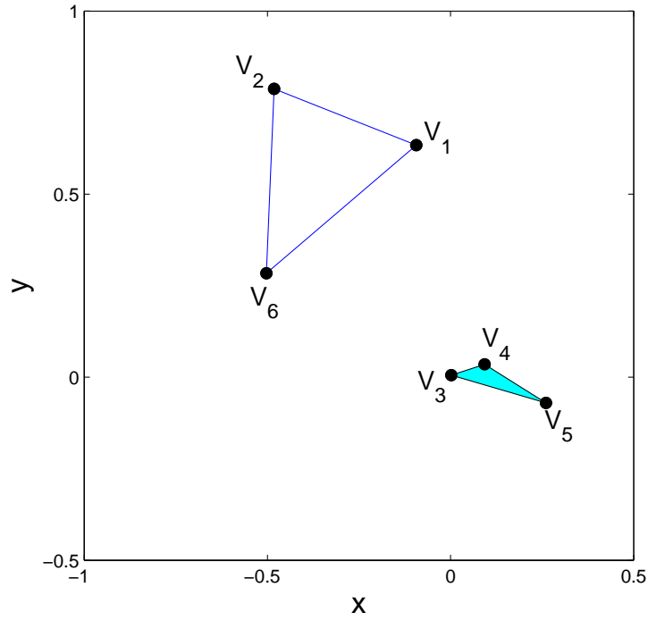
FIG 18. Alpha complex corresponding to the vertex set in Table 7 and r = \sqrt{0.075} .
