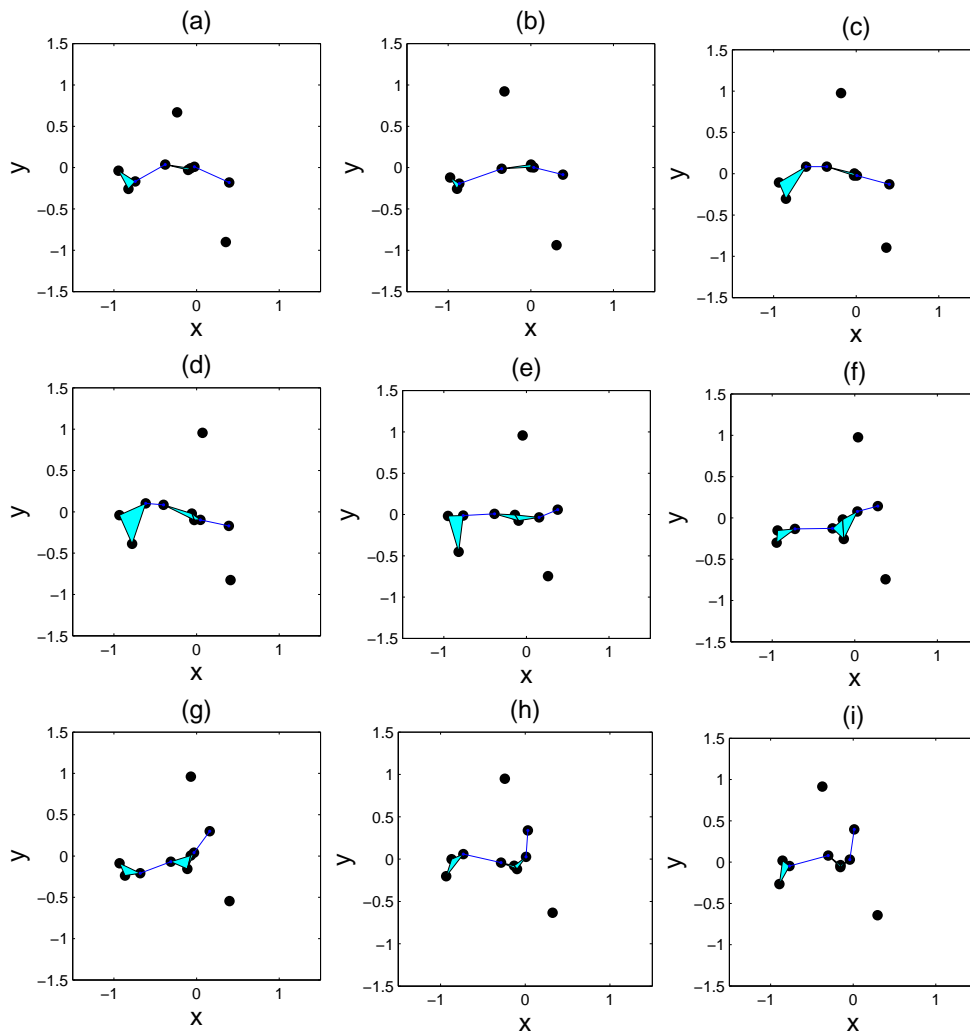
FIG 15. Geometric graphs corresponding to snapshots of posterior samples (one every 100 iterations) from model of (5.1a). For this example graphs are constructed to be decomposable and the clique marginals are specified as Clayton copulas.
