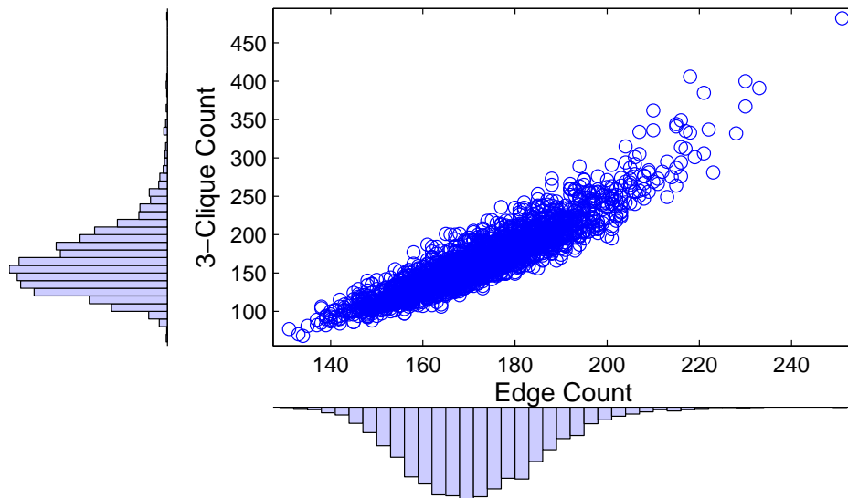
FIG 9. Edge counts and 3-Clique counts from 2,500 simulated samples of \mathcal{G}(\mathbf{V}, 1/\sqrt{2} \cdot 75, \check{C}ech) where |\mathbf{V}| = 75 and V_i \stackrel{iid}{\sim} Un([0, 1]^2) , 1 \leq i \leq 75 . The multivariate normal appears as a reasonable approximation for the joint distribution, as suggested by [25, Thm. 3.13]. Čech radius is r_n = 1/\sqrt{2n} .
