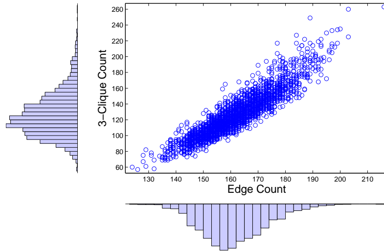
FIG 10. Edge counts and 3-Clique counts from 2,500 simulated samples of \mathcal{G}(\mathbf{V}, 1/\sqrt{2} \cdot 75, \check{C}ech) where |\mathbf{V}| = 75 and V sampled from a Matérn III with hard-core radius r = 0.35 .
