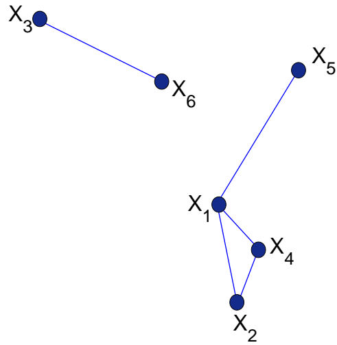
FIG 16. Graph encoding the Markov structure of the model given by precision matrix (5.3).
