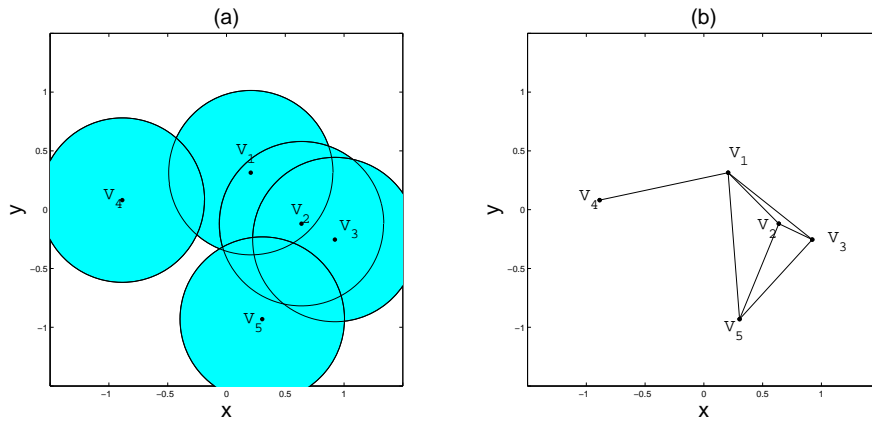
FIG 5. (a) Čech complex computed using r = 0.7 and the vertex set listed in Table 1. (b) The 1-Skeleton of the Čech complex.
