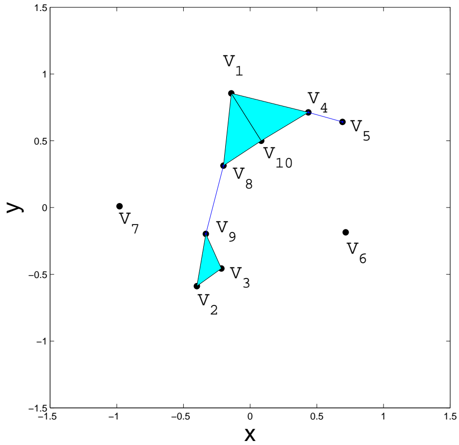
FIG 14. Geometric graph representing the model given in (5.1a). For this example graphs are constructed to be decomposable and the clique marginals are specified as Clayton copulas.
