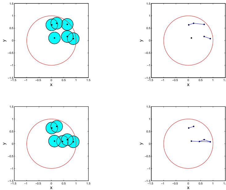
FIG 13. This figure illustrates a local move. (a) The current configuration of the points. (b) The graph implied by this configuration. (c) The proposal configuration which is obtained by randomly moving one vertex. (d) The graph implied by the proposed move.
