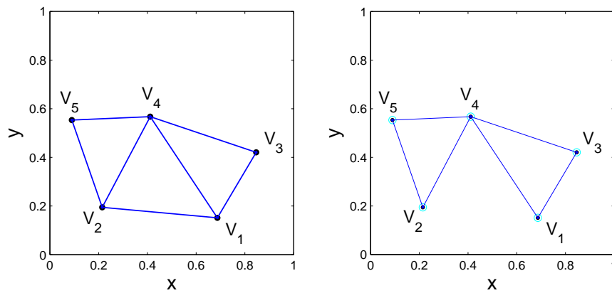
FIG 7. (a) Proximity graph computed from the vertex set given in Table 2. (b) The decomposable graph computed from the same vertex set using Algorithm 1. The edge (1,2) is not included in the decomposable graph.
