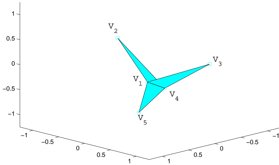
FIG 20. Graph encoding the Markov structure of the model given in (5.6).
