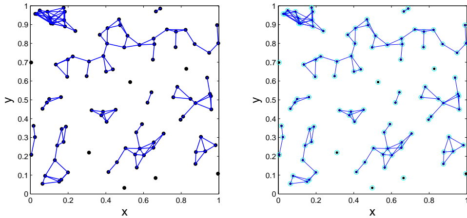
FIG 8. (a) The 1-Skeleton of Čech complex given the displayed point set and r = 0.05 . (b) The decomposable graph for the same complex, point set, and radius output by Algorithm 1.
