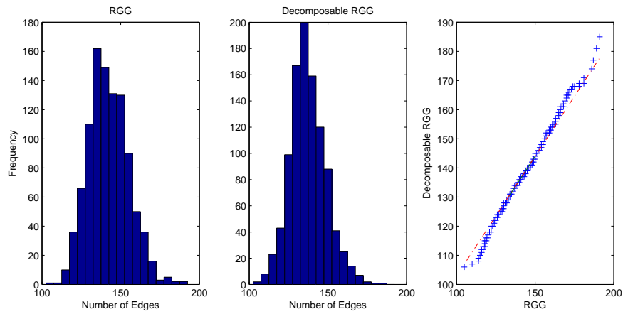
FIG 12. Distribution of edge counts for both unrestricted and decomposable graphs. Graphs were computed using Čech complex filtrations with n = 100 and V_i \stackrel{iid}{\sim} Un([0, 1]^2) .
