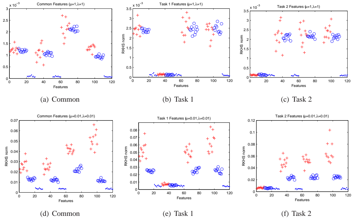
Figure 2: Variance-bias tradeoff and regularization. [a,b,c] \mu, \lambda = 1 . [d,e,f] \mu, \lambda = .01 . High variance features in red, low variance features in blue.
