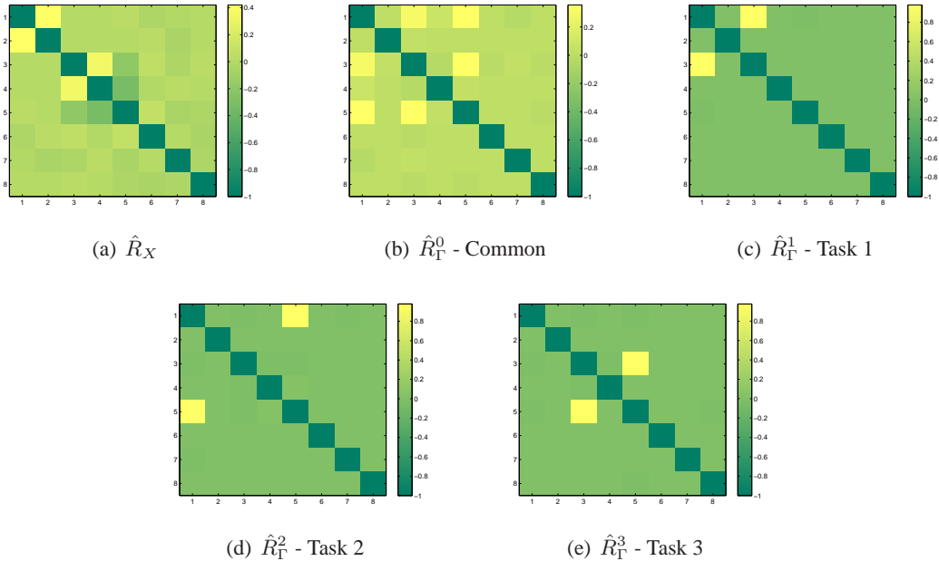
Figure 5: Conditional Dependence Simulation (a) Partial correlation of data matrix X. (b-e) Partial correlation matrices using gradient outer products.
