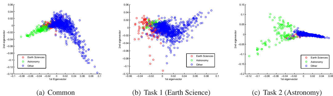
Figure 4: Earth Sciences & Astronomy vs Other. Plots depict corresponding embedding of data using top 2 eigenvectors.
