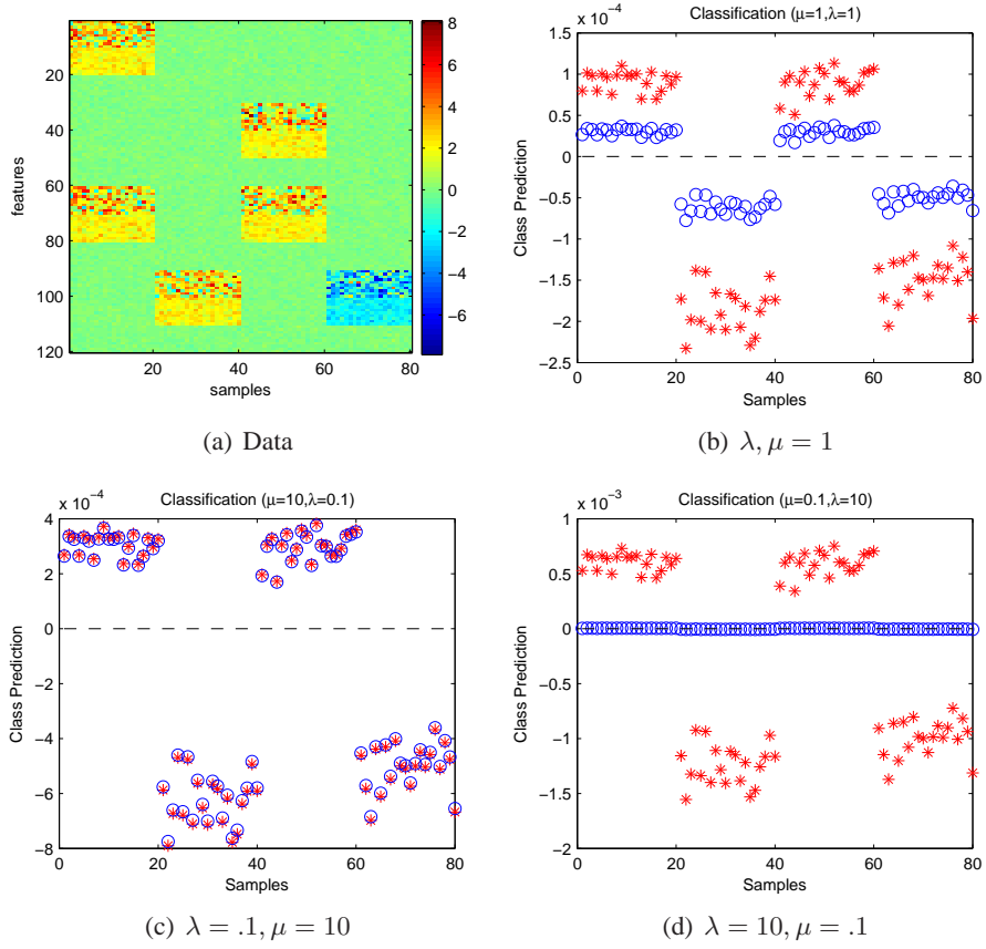
Figure 1: (a) Data matrix x , column samples; samples 1 \dots 20 correspond to task 1, class +1; samples 21 \dots 40 , task 1, class -1; samples 41 \dots 60 task 2, class +1; samples 61 \dots 80 task 2, class -1, (b,c,d) F_t (blue) and f_t (red) using different regularization parameters.
