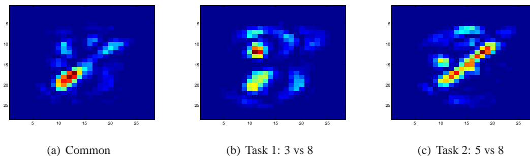
Figure 3: Digit plots of the top eigenvectors after a decomposition of the common, task 1, and task 2 GOP matrices.
